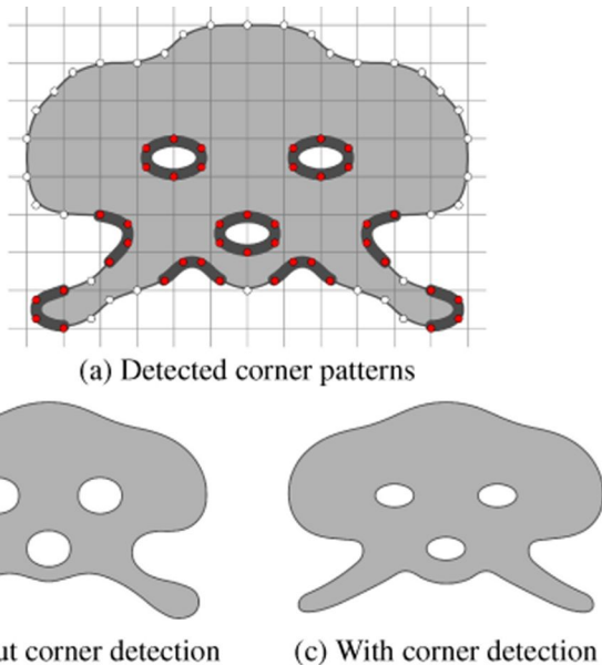
Figure 8: Corner detection: (a) Nodes that belong to a detected corner pattern are shown in red. The curve segments excluded from the evaluation of the smoothness term are highlighted in black.
