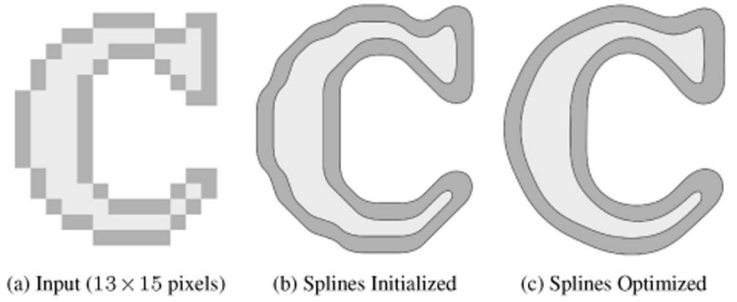
Figure 6: Removing staircasing artifacts by minimizing spline curvature.
