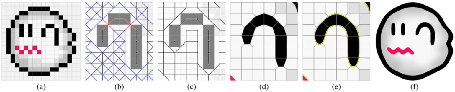
Figure 3: Overview of our algorithm. (a) Input Image ( 16 \times 16 pixels). (b) Initial similarity graph with crossing edges. The blue edges lie inside flat shaded regions, so they can be safely removed. In case of the red lines, removing one or the other changes the result. (c) Crossing edges resolved. (d) Reshaped pixel cells reflecting the connections in the resolved similarity graph. (e) Splines fit to visible edges. (f) Final result with splines optimized to reduce staircasing (Image © Nintendo Co., Ltd.).
