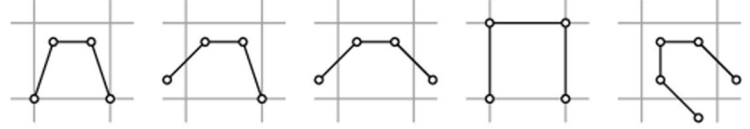
Figure 7: Corner patterns our algorithm detects. The original square pixel grid is shown in gray. Detecting these patterns is straight forward because node locations are quantized to multiples of a quarter pixel in both dimensions due to the graph construction.
