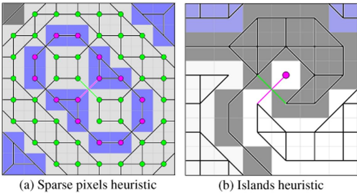
Figure 4: Heuristics for resolving crossing edges in the similarity graph: Curves: not shown here, see Figure 3b. Sparse pixels: the magenta component is sparser than the green one. This heuristic supports keeping the magenta edge connected. Islands: In this case the heuristic supports keeping the magenta edge connected, because otherwise a single pixel “island” would be created.
